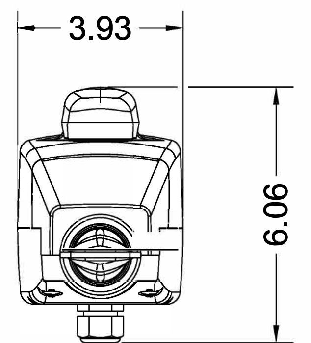
RIGHT VIEW
