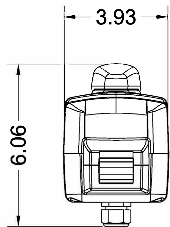
LEFT VIEW
