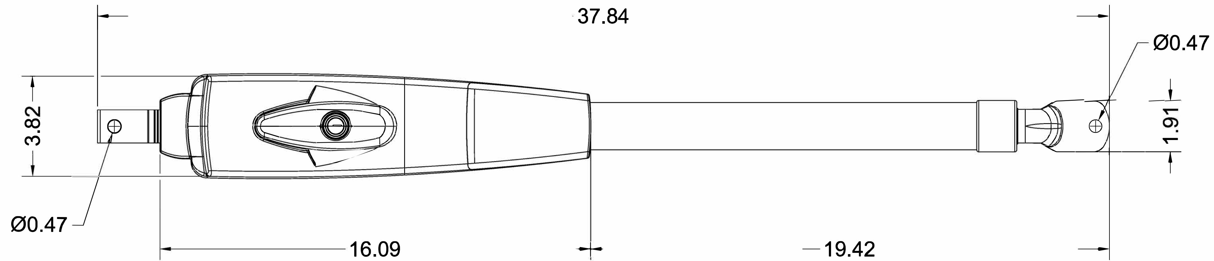
TOP VIEW
