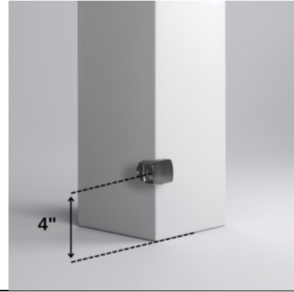
Mounting Position for Overhead Doors
