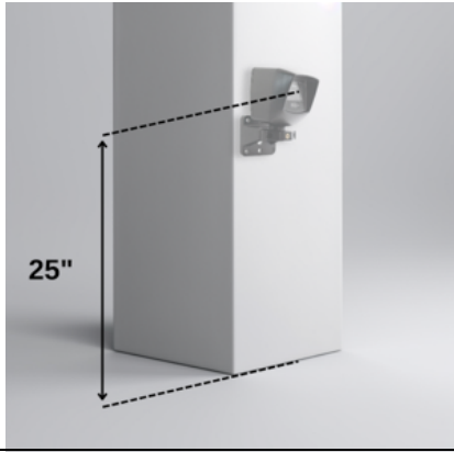
Mounting Position for Gates
