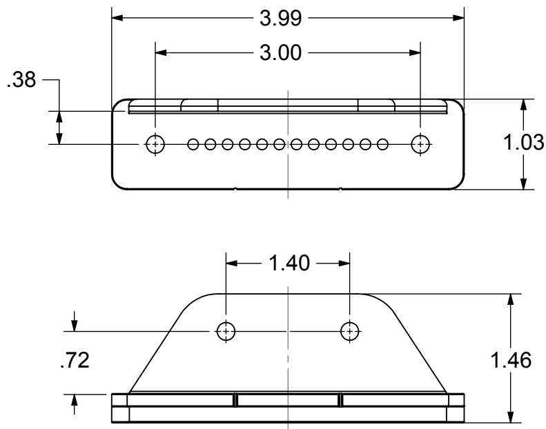
LOWER MOUNTING BRACKET
